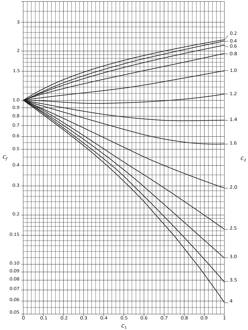
Figure 26-5 Coefficient C_f
