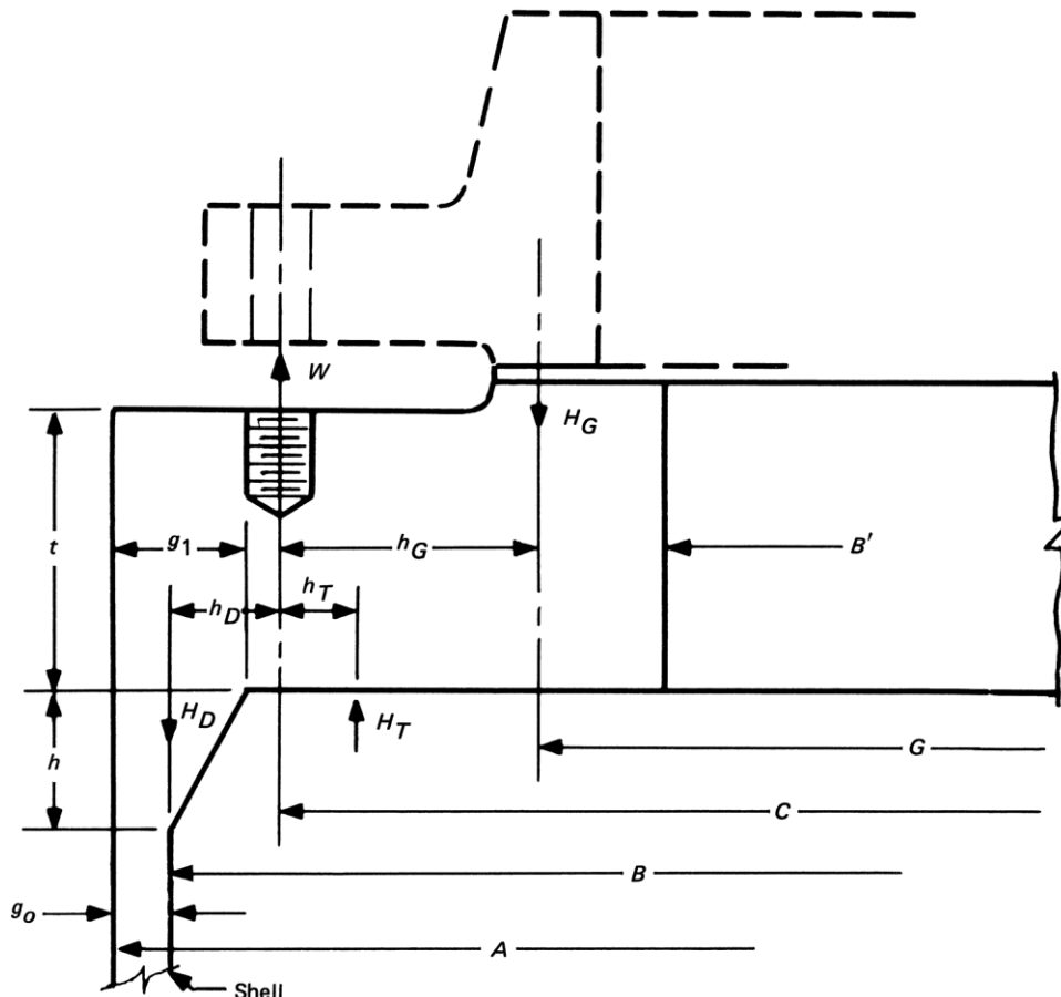
Figure 2-13.1 Reverse Flange
