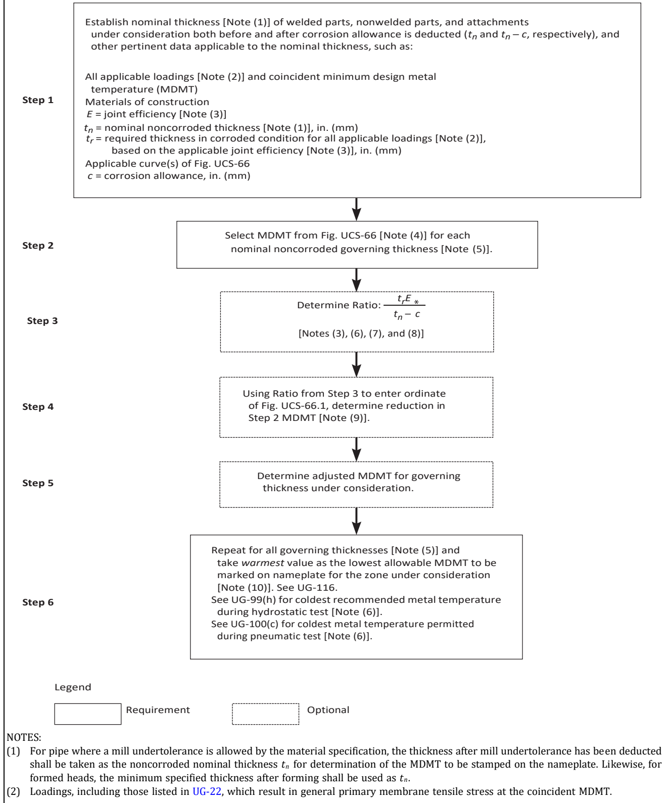
Figure UCS-66.2 Diagram of UCS-66 Rules for Determining Lowest Minimum Design Metal Temperature (MDMT) Without Impact Testing
