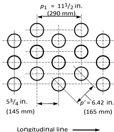
Figure UG-53.4 Example of Tube Spacing With Tube Holes on Diagonal Lines
