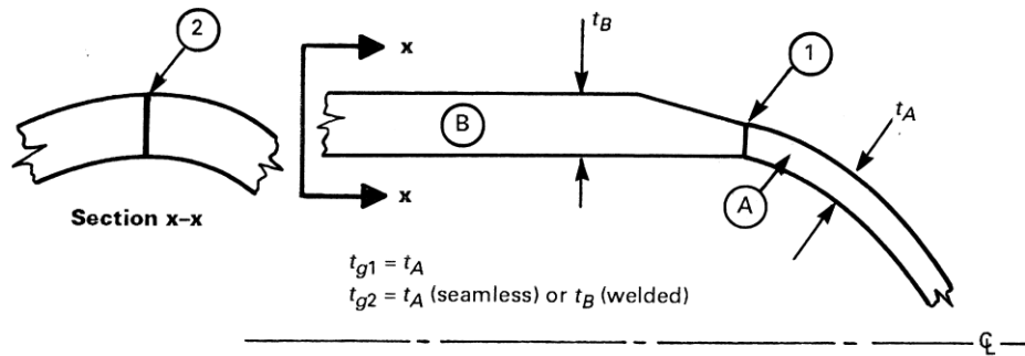
(a) Butt Welded Components
