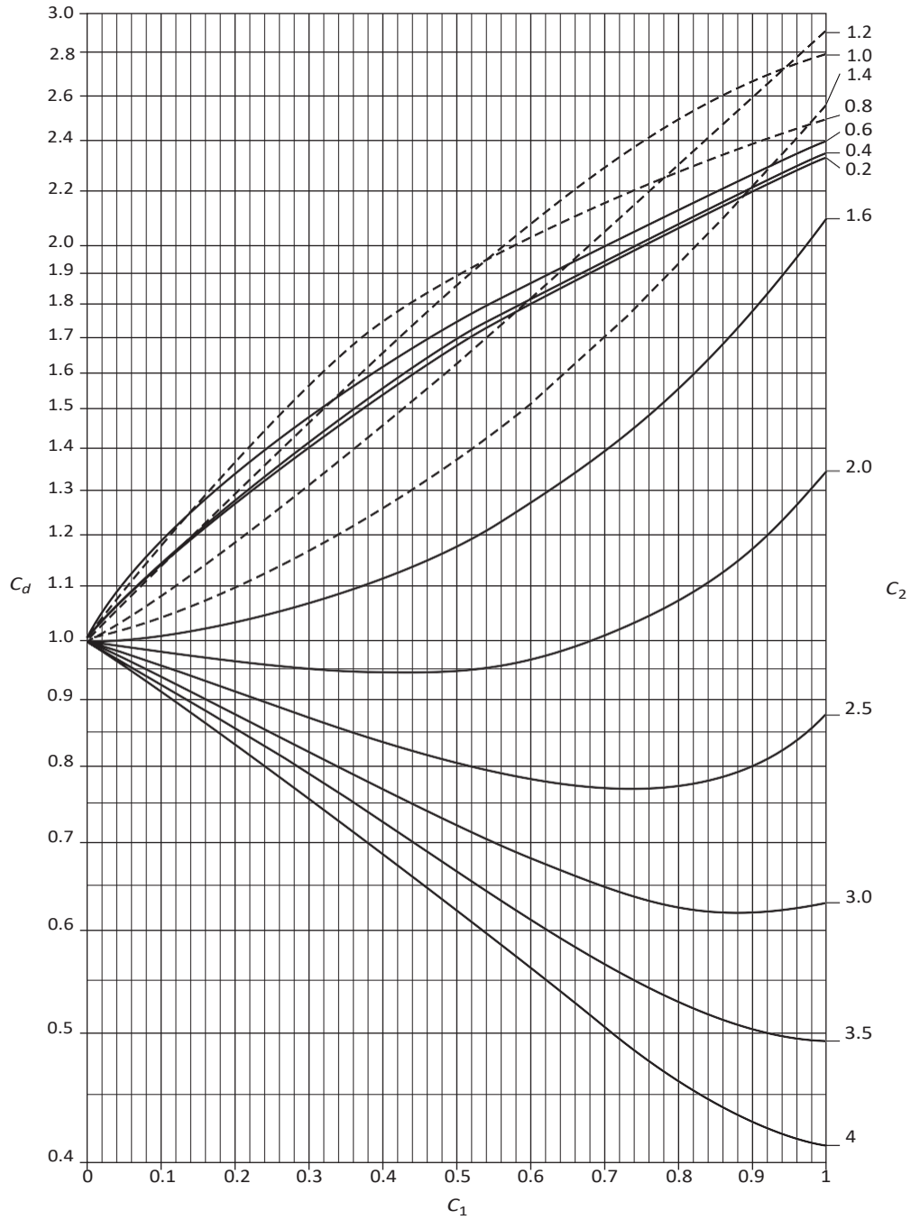
Figure 26-6 Coefficient C_d
