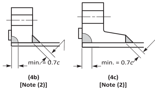
Loose-Type Flanges [Notes (3) and (4)]
